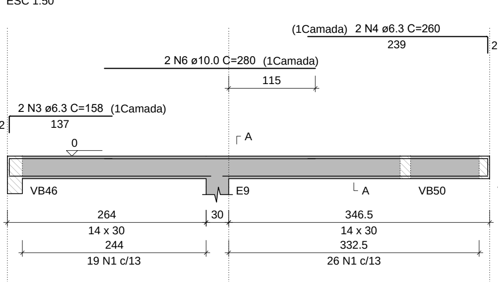
VB12 (14 x 30)
